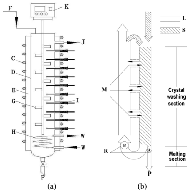
Fig. 2. (a) Schematic diagram of experiment setup. (b) Schematic of stream flow in the crystallization column.
